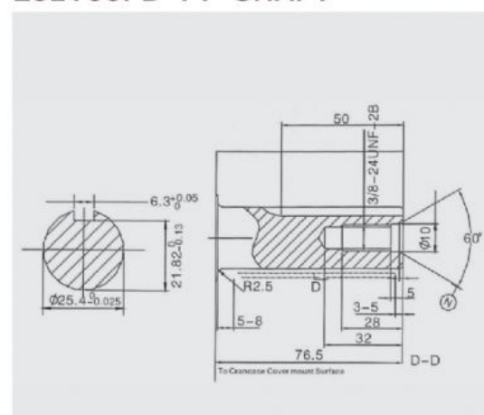
LC2V80FD-1 P-SHAFT
