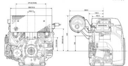
HIGH MOUNT MUFFLER TYPE
