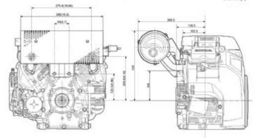
HIGH MOUNT MUFFLER TYPE
