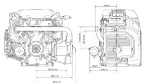
SIDE MOUNT MUFFLER TYPE
